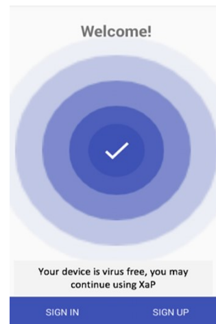
Figure 6: Malware scan
